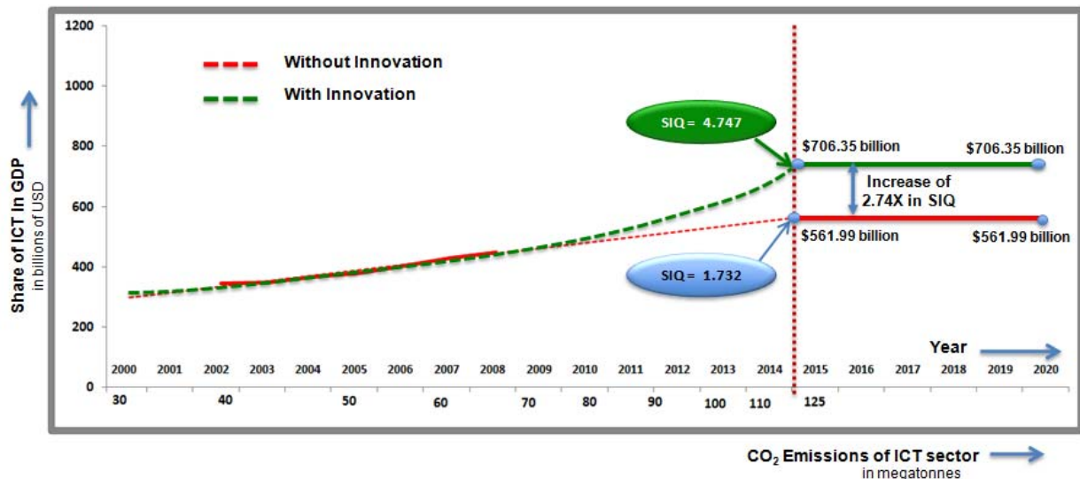
Figure 3: Scenario when ICT's carbon emissions are frozen at 117.5Mt for the United States and the value of Innovation to improving ICT
